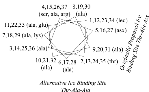
FIGURE 1 Helical wheel representation of the protein. This representation shows the i, i + 11 repeat of the protein. The residue numbers are marked along with the residue composition. The originally proposed Thr-Ala-Asx "ice-binding" face is shown at right, whereas the newly proposed Thr-Ala-Ala face is shown at the bottom.
