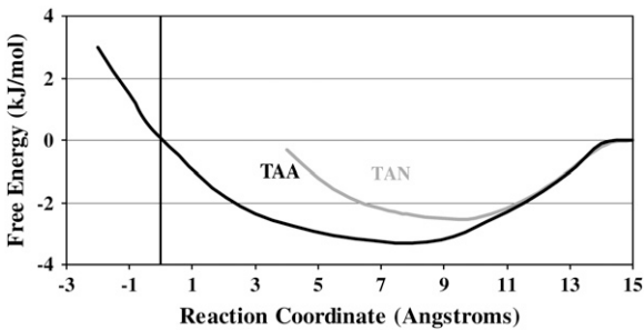
FIGURE 4 Potential of mean force profile. This figure shows the potential of mean force profile, i.e., free energy, of the proteins as a function of distance from the midpoint of the ice/water face. The x axis represents the distance between the center of the protein helix and the midpoint of the ice/water interfacial region. The midpoint of the interfacial region is defined by the inflection point of the diffusion coefficient profile (43). The y axis represents the free energy of interaction between the protein and the ice/water interfacial region in kJ/mol. The free energy of interaction between the protein and bulk water is set at the reference value of 0 kJ/mol.
